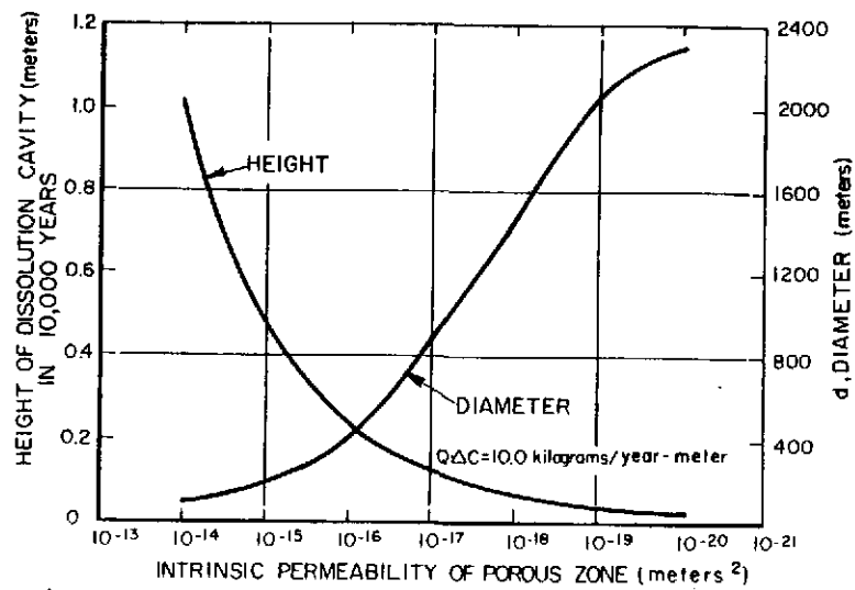
(A) POTENTIAL CAVITY SIZE AS A FUNCTION OF INTRINSIC PERMEABILITY
