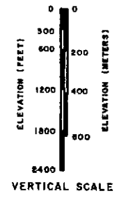
FIGURE 2-1 SITE STRATIGRAPHIC COLUMN PREPARED FOR WESTINGHOUSE ELECTRIC CORPORATION ALBUQUERQUE, NEW MEXICO
