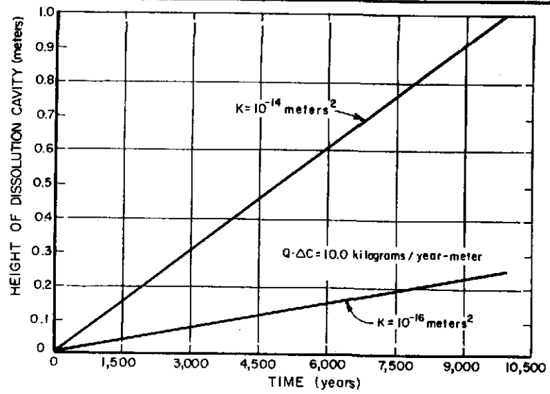
(C) GROWTH OF CAVITY WITH TIME
